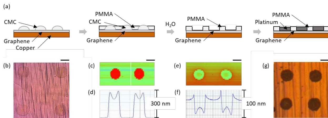
Figure 3. (a) Schematic illustration of the inversion-moulding process that patterns Pt arrays on top of monolayer CVD-graphene sheets. (b) Optical micrograph of the inkjet printed CMC/graphene/Cu array. Scale bar, 20 \mu\text{m} . (c) Vertical profile map of the CMC-PMMA/graphene/Cu array. Scale bar, 20 \mu\text{m} . (d) Linear scan of the vertical profile for the CMC-PMMA/graphene/Cu array. (e) Vertical profile map of the PMMA/graphene/Cu well array. Scale bar, 20 \mu\text{m} . (f) Linear scan of the vertical profile for the PMMA/graphene/Cu well array. (g) Optical micrograph of the electroplated Pt/graphene/Cu array. Scale bar, 20 \mu\text{m} .
