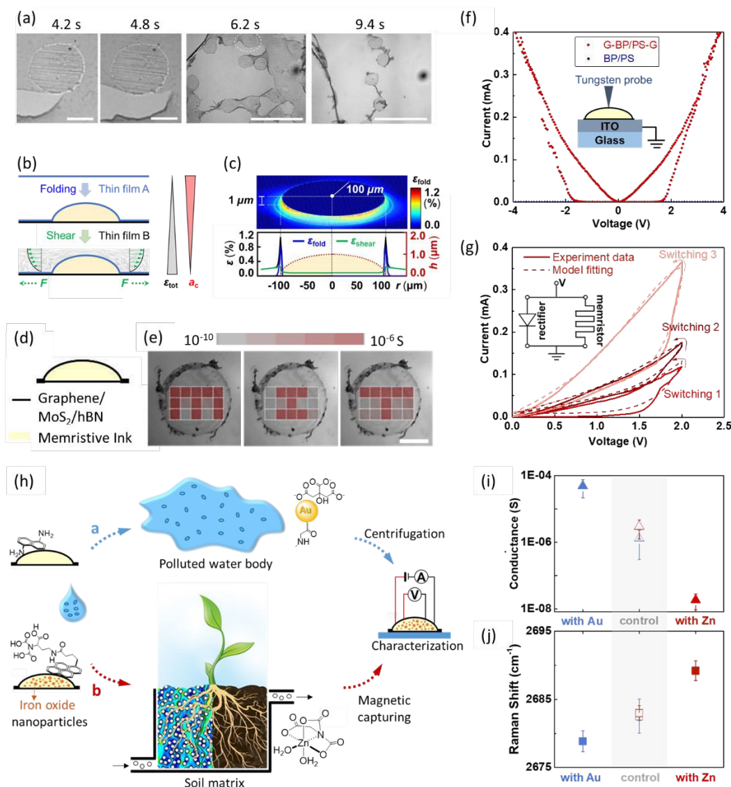
Figure 2. Autoperforated Colloidal State Machines enabled by 2DMs. (a) Optical micrographs of the bottom-up autoperforation technique showing the crack propagation in progress 22 . The round shapes correspond to inkjet-printed discs which impose strains. Scale bars represent 100, 100, 1000, and 1000 \mu\text{m} . (b) Schematic illustration of the two-step process generating the strain field used in (a). The first step involves folding the graphene-containing thin film A on top of the curved polymer disk printed onto film B, which has the same composition as A. The second shearing step is facilitated by flowing an agitated liquid over the film-encapsulated disk, creating a tensile stress within both films synergistic to the folding strain, modelled here as an outward-facing force F pulling uniformly away from the film centre. The total strain ( \epsilon_{\text{tot}} ) within the films increases as a result of this two-step process. The Griffith length ( a_c ), on the other hand, decreases. (c) Local strain field after stacking/folding a thin polymer film (200 nm) onto a microdisk (radius:height = 100:1) based on finite-element analysis. (d) Schematic of the sandwich CSM carved out by the crack "scissors", equivalent to an intraparticle vertical memristor array in parallel. The conductivity map in (e) shows that each of these memristors can be switched on independently, thus mapping out letters "M", "I", and "T". Scale bar, 100 \mu\text{m} . (f) Cross-plane I-V curves of microparticles G-BP (0.9 wt%)/PS-G, G-PS-G, and BP/PS. (g) I-V curves of three successive sweeps of 0 \rightarrow 2 \rightarrow 0
