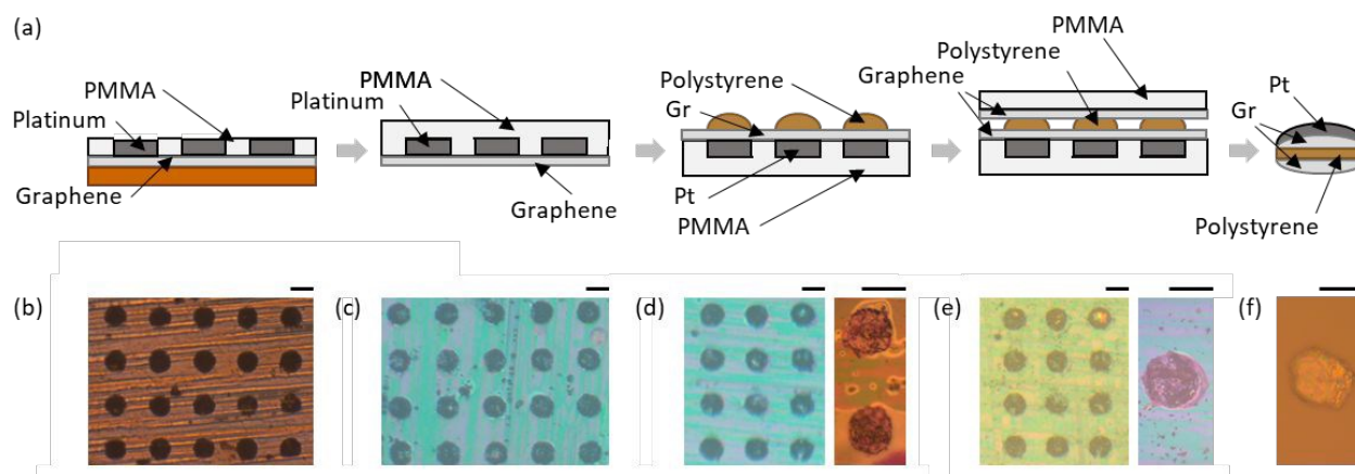
Figure 6. (a) Schematic illustration of the alignment, inkjet printing, and autoperforation process that produces Pt-coated graphene-CSMs in solution. (b) Optical micrograph of the electroplated Pt/graphene/Cu array. Scale bar, 20 \mu\text{m} . (c) Optical micrograph of the spin-coated PMMA/Pt/graphene array with Cu etched away. Scale bar, 20 \mu\text{m} . (d) Optical micrographs of the inkjet printed polystyrene aligned over the PMMA/Pt/graphene array. Scale bars, 20 \mu\text{m} . (e) Optical micrographs of the PMMA/graphene encapsulated polystyrene-PMMA/Pt/graphene array. Scale bars, 20 \mu\text{m} . (f) Optical micrographs of the autoperforated Pt-coated graphene-CSM (Pt/graphene/polystyrene/graphene) dried on a glass slide. Scale bar, 20 \mu\text{m} .
