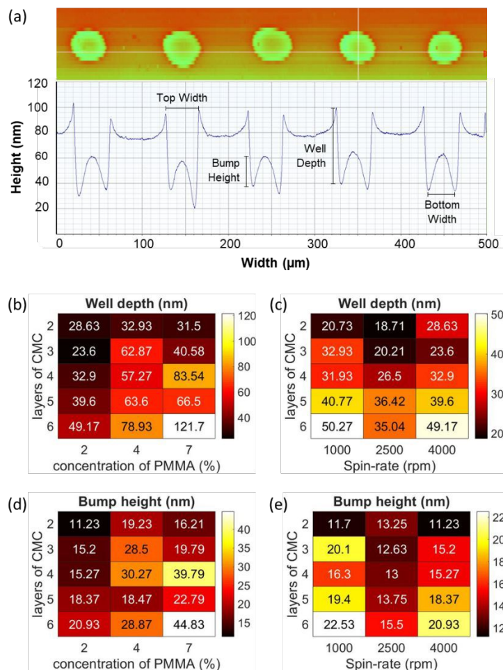
Figure 5. (a) Example of profilometer dimensions of interest from a linear scan. The dimensions of interest include the width at the top and bottom of the well, the well depth, and the height of the bump formed at the base of each well. Inset, example of 2D height profile of PMMA wells. (b-e) Summary data for profilometer measurements of the PMMA wells. The heat maps show well depth as a function of (b) layers of CMC and concentration of PMMA, (c) layers of CMC and spin-rate, as well as bump height as a function of (d) layers of CMC and concentration of PMMA, (d) layers of CMC and spin-rate.
