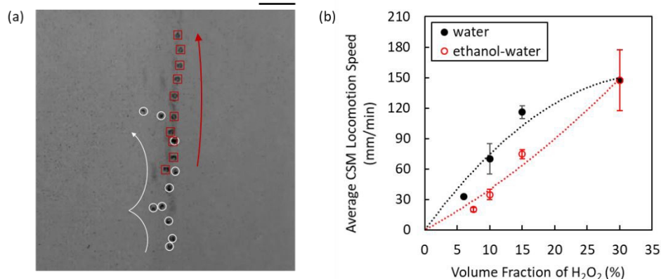
Figure 7. (a) Superimposed images of sequential frames show the locomotion of two Pt/graphene-CSMs (white circles and red squares). Arrows indicate the migration direction. Scale bar, 100 \mu\text{m} . (b) Averaged CSM translocation speed for Pt/graphene-CSMs in 30 volume percent \text{H}_2\text{O}_2 aqueous solution diluted using water (black) or ethanol (red). Data averaged from two experiments and the error bars represent their deviation. The dashed lines are guide for the eye. For ethanol-diluted solution, the volumetric ratios of ethanol:water solution used are (from left to right): 3:1, 2:1, 1:1, 0.
